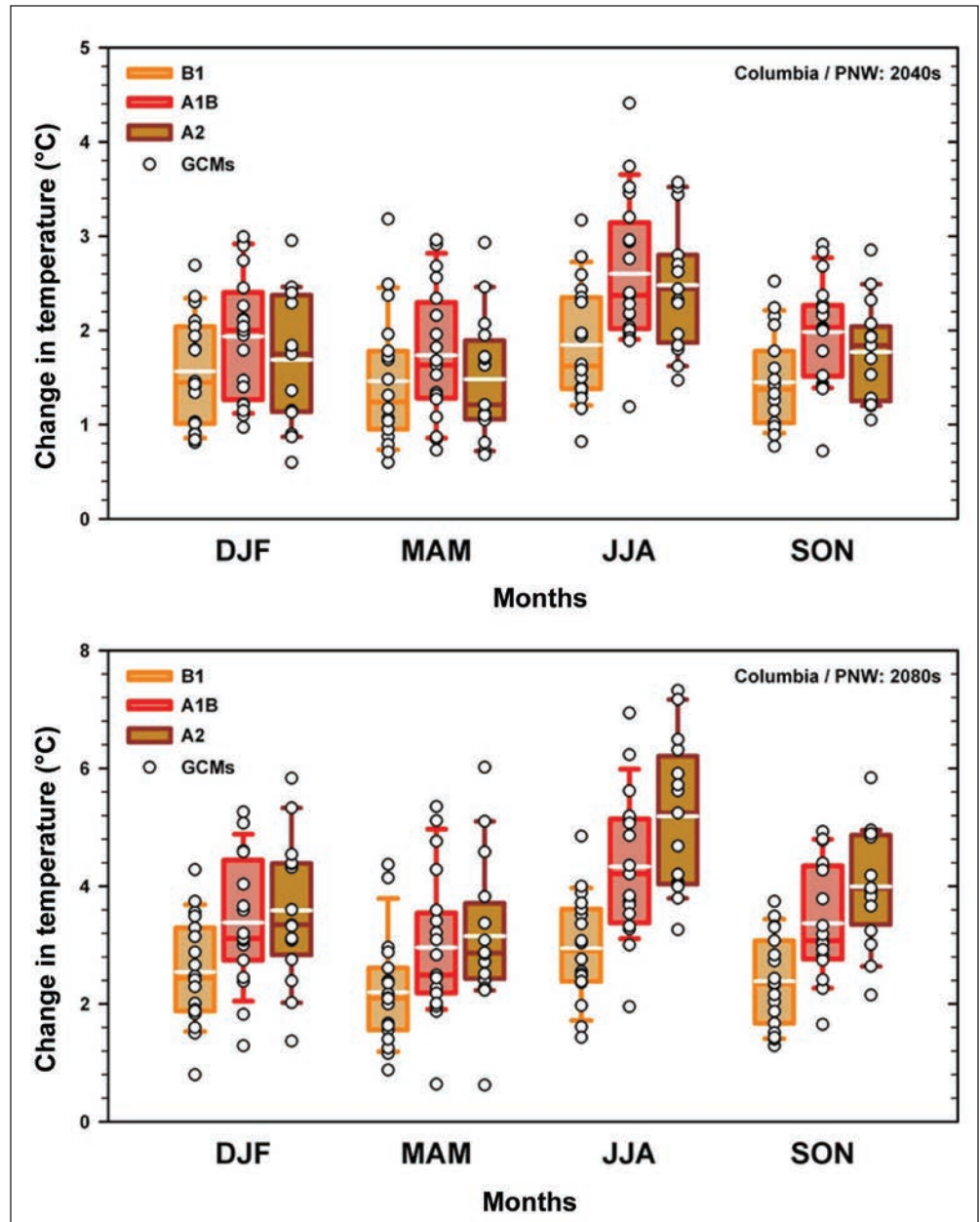
Figure 3.3—Range of projected changes in temperature (relative to 1970–1999) for the Columbia River basin/Pacific Northwest for the 2040s (top) and 2080s (bottom) for each season (letters indicate first letter of the month). In each box-and-whisker trio, the leftmost is for emissions scenario B1, center for A1B, and right for A2; circles are individual model values. Box-and-whisker plots indicate 10 th and 90 th percentiles (whiskers), 75 th percentiles (box ends), and median (solid middle bar) for each season and scenario. White bars indicate mean of deltas for global climate models. (Data source: Littell et al. 2011.)
