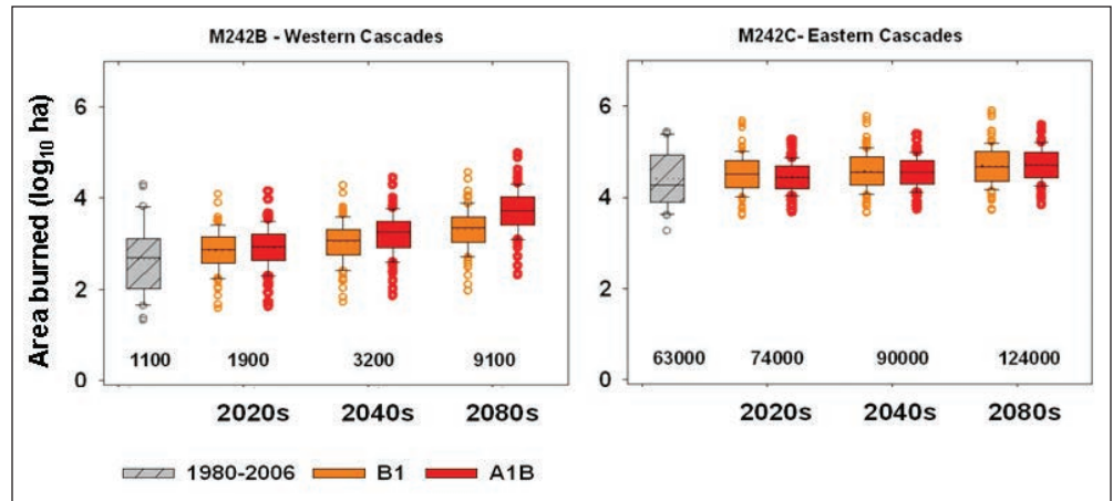
Figure 5.11—Expected changes in area burned for scenarios of future climate and hydrology in the western and eastern Cascades (Bailey ecosections). The B1 scenario represents less warming with lower greenhouse gas emissions. The A1B scenario represents more warming with higher greenhouse gas emissions, and is the highest average of the SRES scenarios until the 2040s. The area burned in both ecosections increases substantially, but the rate of increase is higher in the western Cascades than the eastern Cascades. Numbers beneath the box indicate the average annual area burned for the historical period and three future periods (Littell et al. 2010).
