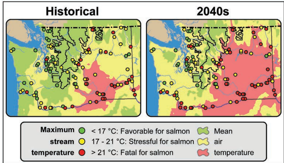
Figure 7.4—Color shading shows mean surface air temperatures for August, and shaded circles show the simulated mean of the annual maximum for weekly water temperatures (average, not transient) at select locations. Historical (1970–1999) reference period data are in the left panel, and the average future scenario for an ensemble of 10 global climate models under the A1B emissions scenario for the 2040s is shown in the right panel. The color scheme used here is tailored to three general categories for thermal rearing habitats for salmonids: greens indicate favorable, yellows indicate stressful, and reds indicate fatal.
