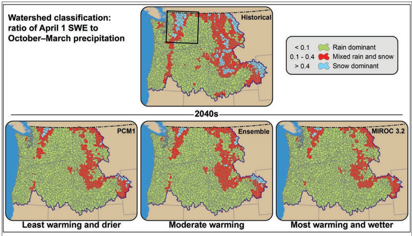
Figure 4.2—Projected shift in watershed basin type in the Pacific Northwest by the 2040s (2030–2059). Basins represent the spatial resolution of 10-digit hydrologic unit codes (HUCs), or the 5 th -level watershed classification as delineated by the U.S. Geological Survey. Basin types are defined by the ratio of April 1 snow water equivalent (SWE) to cool season (October through March) precipitation, which represents most precipitation falling as snow or rain. Future projections were modeled using the A1B emission scenario and three model configurations, an ensemble of 10 GCMs and two bracketing GCMs (one projecting less warming and drier conditions than the ensemble mean [PCM1] and one projecting more warming and wetter conditions than the ensemble mean [MIROC 3.2]). Black box in first plot is zoomed in on figure 4.3.
