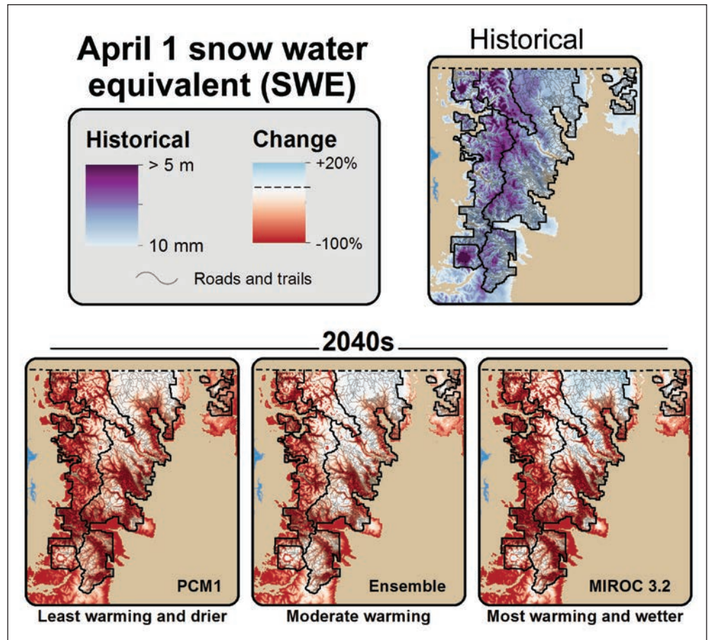
Figure 4.6—April 1 SWE in the North Cascades in the 2040s (2030–2059) shown as a percentage change from historical levels (1916–2006), calculated as ([\text{future} - \text{historical}] / \text{historical}) \times 100 . Percentage change indicates the difference between future projections and historical levels. Future projections were modeled using the A1B emission scenario and three model configurations, an ensemble of 10 GCMs and two bracketing GCMs (one projecting less warming and drier conditions than the ensemble mean [PCM1] and one projecting more warming and wetter conditions than the ensemble mean [MIROC 3.2]). Data are resolved at 30 arc-sec (about 800 m) resolution (see footnote 3).
