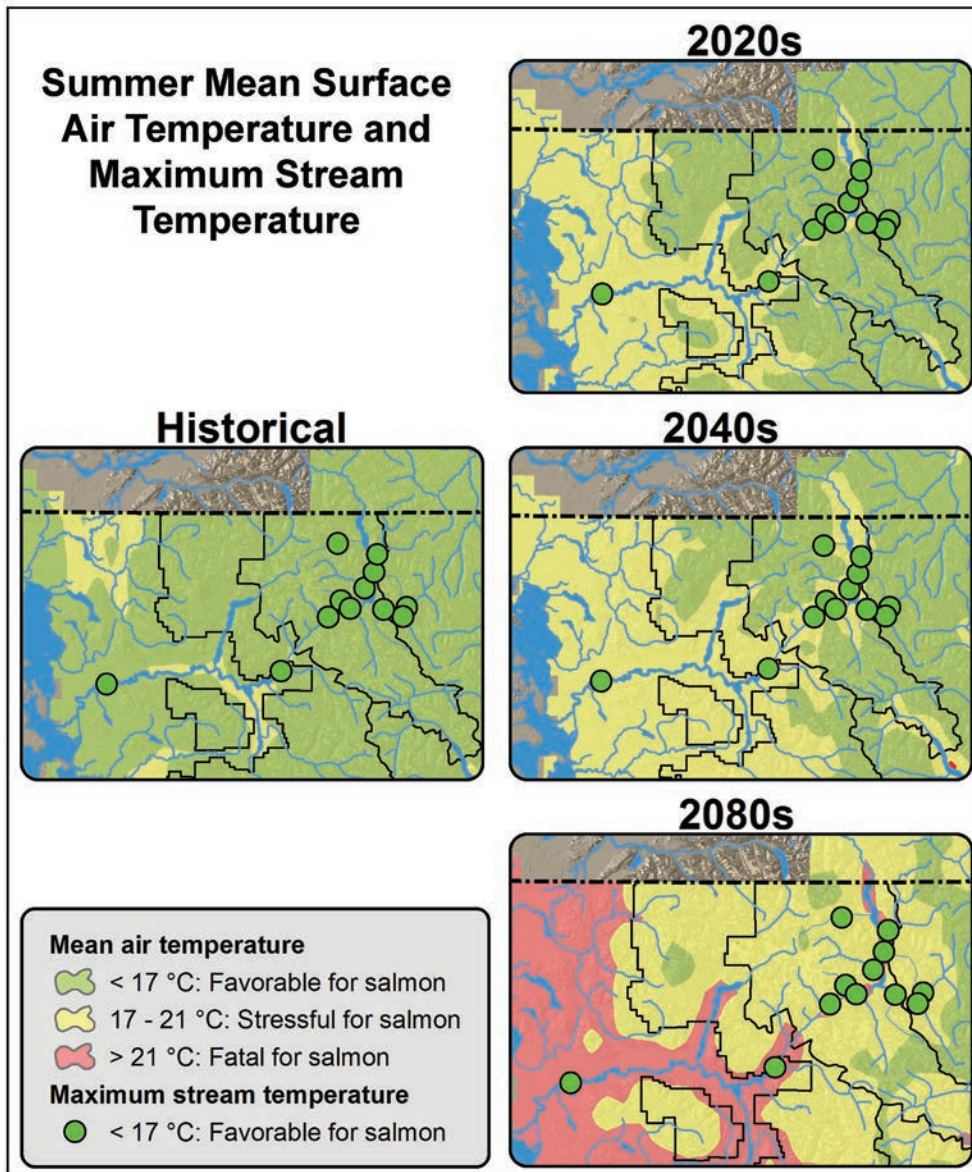
Figure 7.5—August mean surface air temperature and maximum weekly average water temperatures for select locations in the Skagit River basin. The color scheme used here is tailored to three general categories for thermal rearing habitats for salmonids. For mean air temperature, greens indicate favorable, yellows indicate stressful, and reds indicate fatal. The color scheme for stream temperature is associated with criteria for salmonids: green indicates temperatures below 17 °C.
