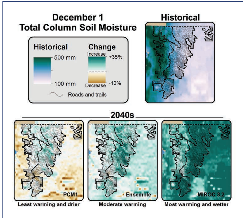
Figure 4.9—Percentage of change in total soil moisture content on December 1 in the North Cascades for the 2040s (2030–2059) compared to historical levels (1916–2006), calculated as (\text{future}/\text{historical}) / \text{historical} \times 100 . Future projections were modeled using the A1B emission scenario and three model configurations, an ensemble of 10 GCMs and two bracketing GCMs (one projecting less warming and drier conditions than the ensemble mean [PCM1] and one projecting more warming and wetter conditions than the ensemble mean [MIROC 3.2]).
