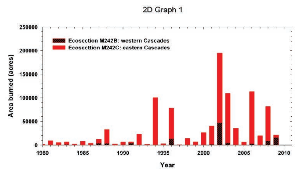
Figure 5.10—Area burned in the western and eastern Cascades (Washington and Oregon), 1980–2009. The data from 2010 were provisional at the time of analysis. Data: Littell and Gwozdz (2011).
