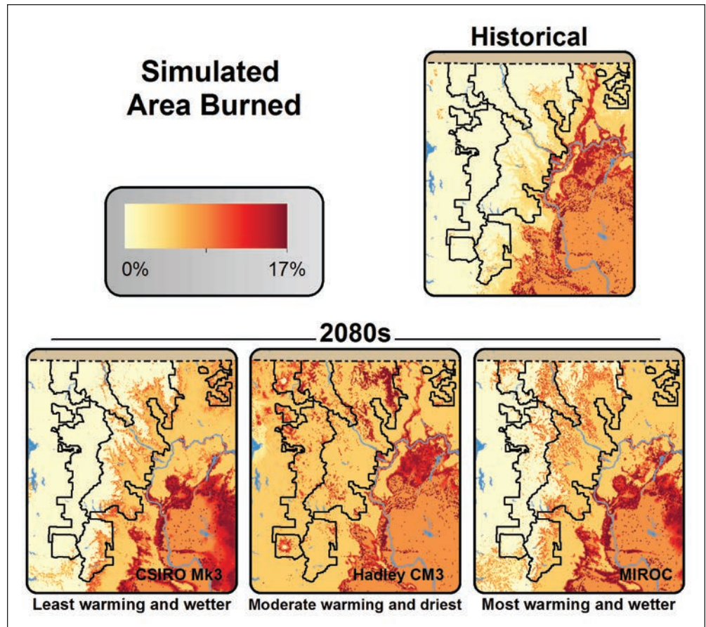
Figure 5.12—Changes in cell fraction area burned from the MCI dynamic global vegetation model. Data: Databasin (Rogers et al. 2011).
