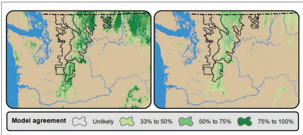
Figure 5.6—Historical (left) and 2060s (2050–2079) changes in climatic suitability for lodgepole pine, based on climate correlations with current species distributions. Data: Rehfeldt et al. (2006), analysis after Littell et al. (2010).
