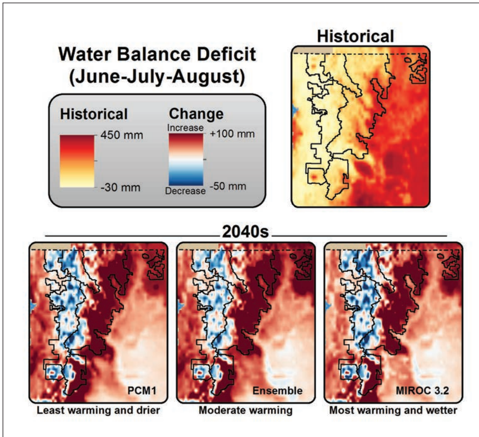
Figure 5.3—Historical (1916–2006) and future (2030–2059, and 2070–2099) June-July-August water balance deficit, adapted from Elsner et al. (2010).
