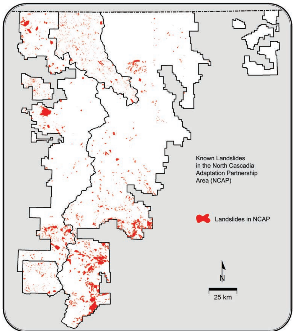
Figure 4.8—Inventoried historical landslides (i.e., mass wasting events) in the North Cascades, 1940–2005. Inventoried landslides include block fall or topple, debris flow, debris slide or avalanche, deep-seated, hyperconcentrated flow, shallow undifferentiated, and unknown type. (Data from the State of Washington, Department of Natural Resources; Mount Rainier National Park; and North Cascades National Park Complex.)
