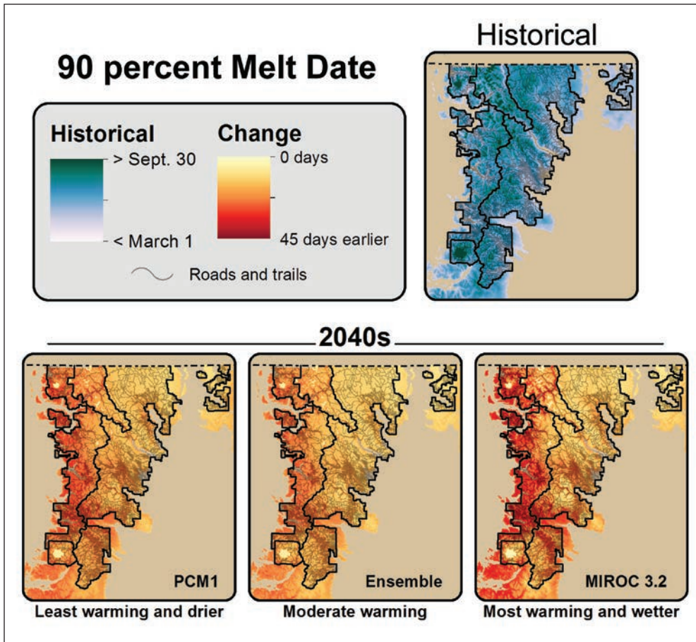
Figure 4.7—Average change in date at which 90 percent of the snow water equivalent is melted for the 2040s (2030–2059) compared to historical dates (1916–2006). Change indicates the difference in number of days between future projections and historical levels. Future projections were modeled using the A1B emission scenario and three model configurations, an ensemble of 10 GCMs and two bracketing GCMs (one projecting less warming and drier conditions than the ensemble mean [PCM1] and one projecting more warming and wetter conditions than the ensemble mean [MIROC 3.2]). Data are resolved at 30 arc-sec (about 800 m) resolution. (see footnote 3).
