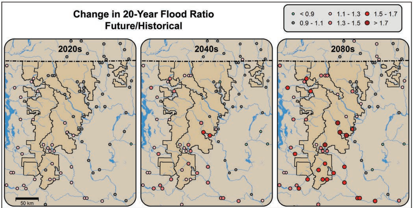
Figure 7.3—Ratio of future to historical simulated 20-year return interval flood statistics, from an ensemble of 10 global climate model simulations under the A1B emission scenario. The left panel is for the 2020s, middle panel is for the 2040s, and right panel is for the 2080s. Figure adapted from Mantua et al. (2010) and data from Hamlet et al. (2010).
