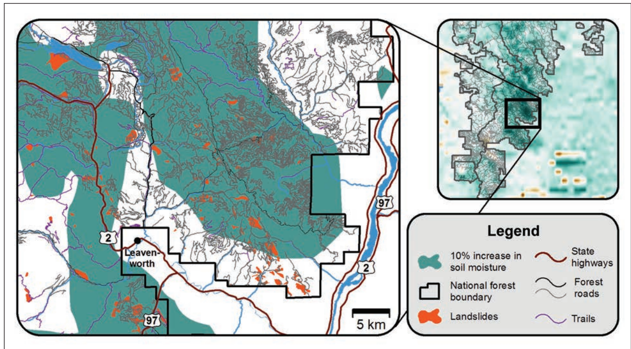
Figure 4.13—An area on the eastern slope of the Cascade Range near Leavenworth, Washington, with more than a 10 percent increase (shown in blue-green) in December 1 total soil moisture projected for the 2040s (2030–2059). This area is shown with known historical landslides. Areas with increases in December 1 total soil moisture may have higher risk of landslides, suggesting locations to prioritize for drainage improvements, rerouting, and road decommissioning. These are also areas where wetter soils may require shifts in trail and road surface and subgrade design and maintenance.
